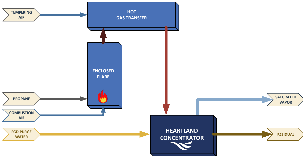
Figure 2. Simplified process flow schematic of the Heartland Concentrator at Power Plant.
