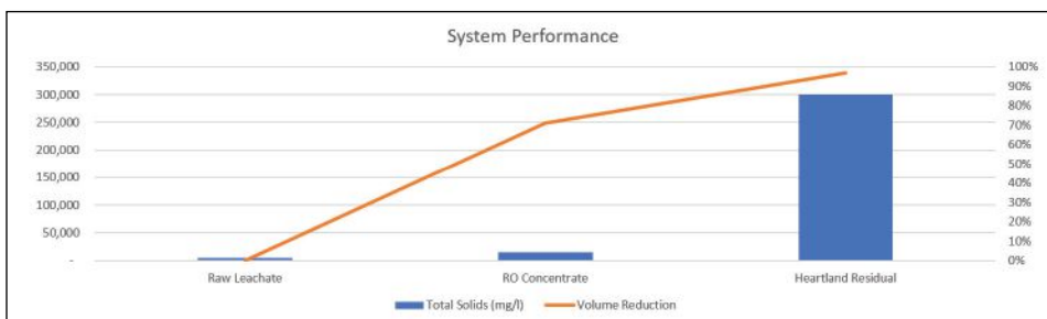
Chart 1. Wastewater Treatment, July-August 2021
