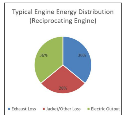
Figure 3. Typical Reciprocating Engine Energy Distribution
